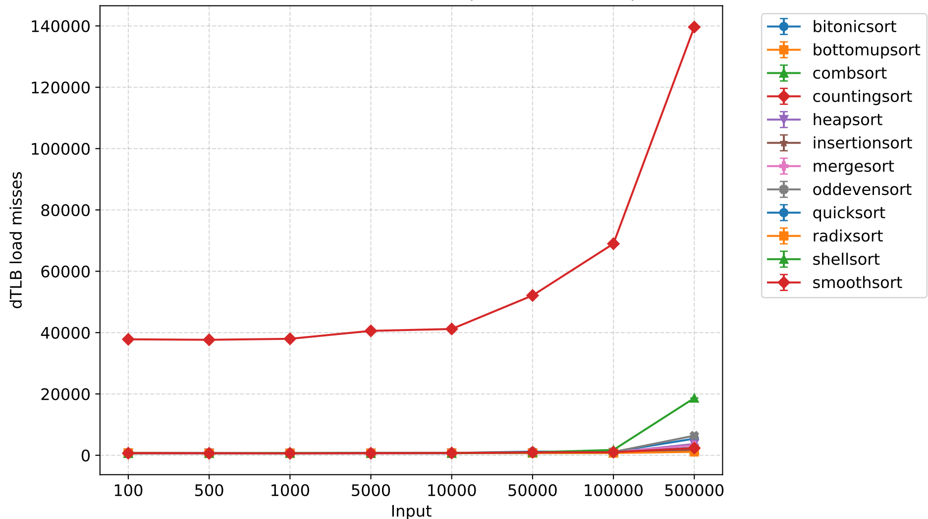
dTLB load misses - 4 threads (mean \pm 95% CI)
