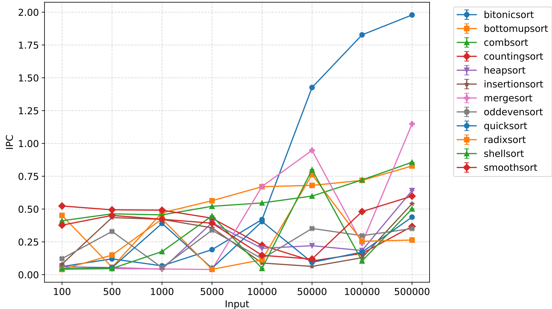
IPC - 4 threads (mean \pm 95% CI)
