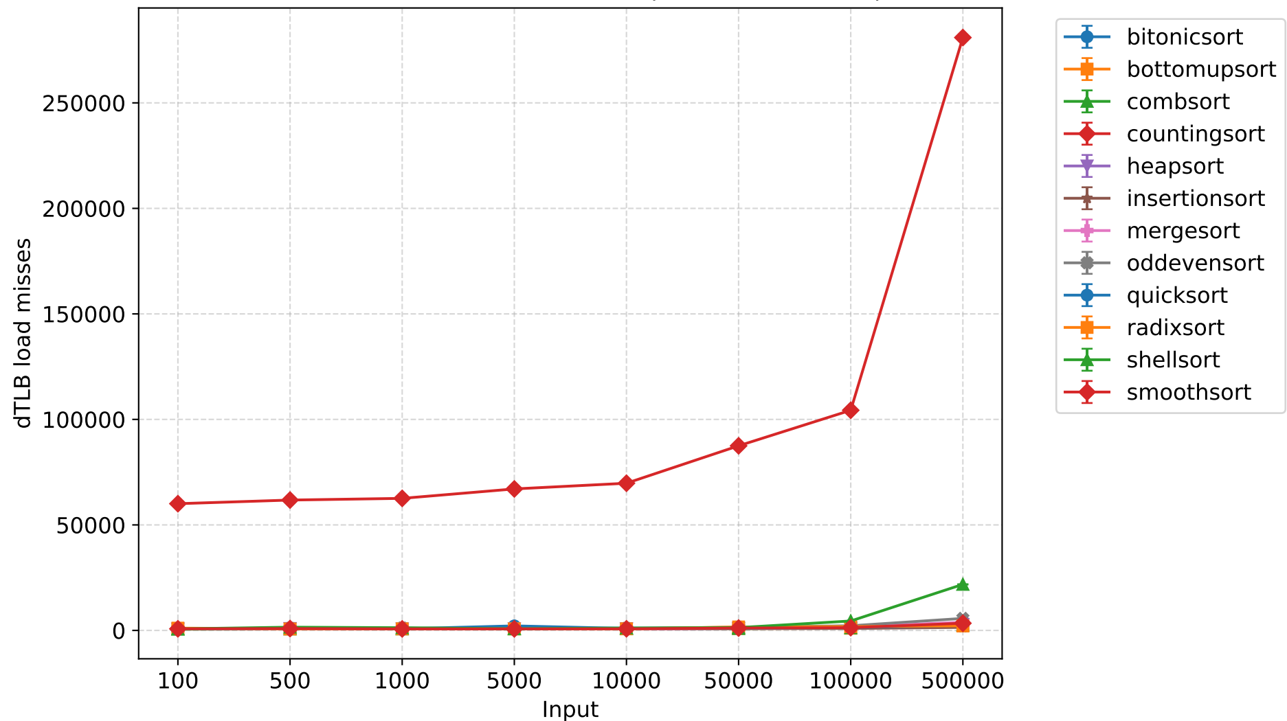
dTLB load misses - 8 threads (mean \pm 95% CI)
