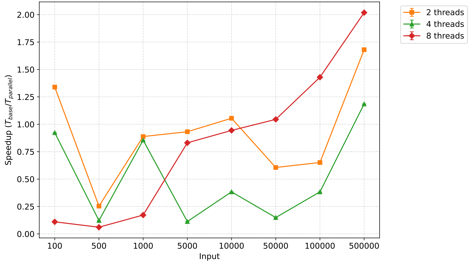
Speedup - insertionsort (mean +- 95% CI)
