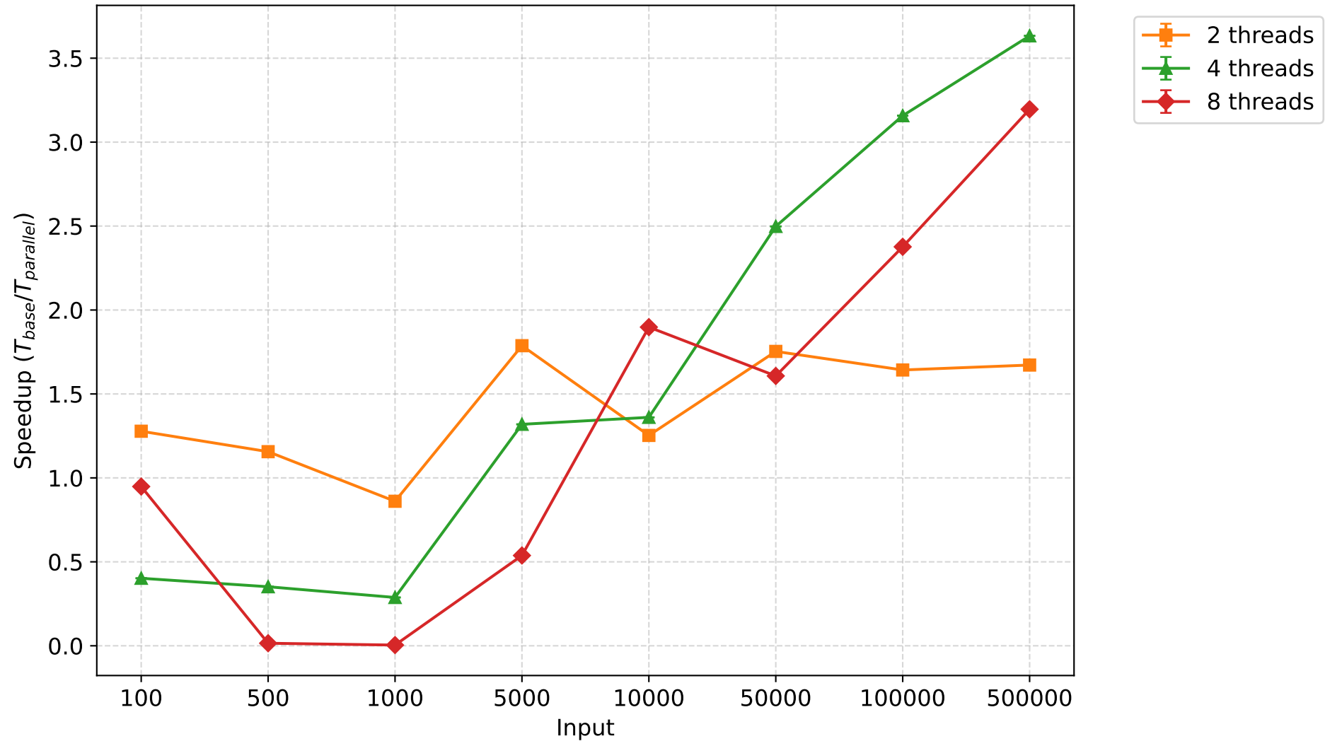
Speedup - oddevensort (mean \pm 95% CI)
