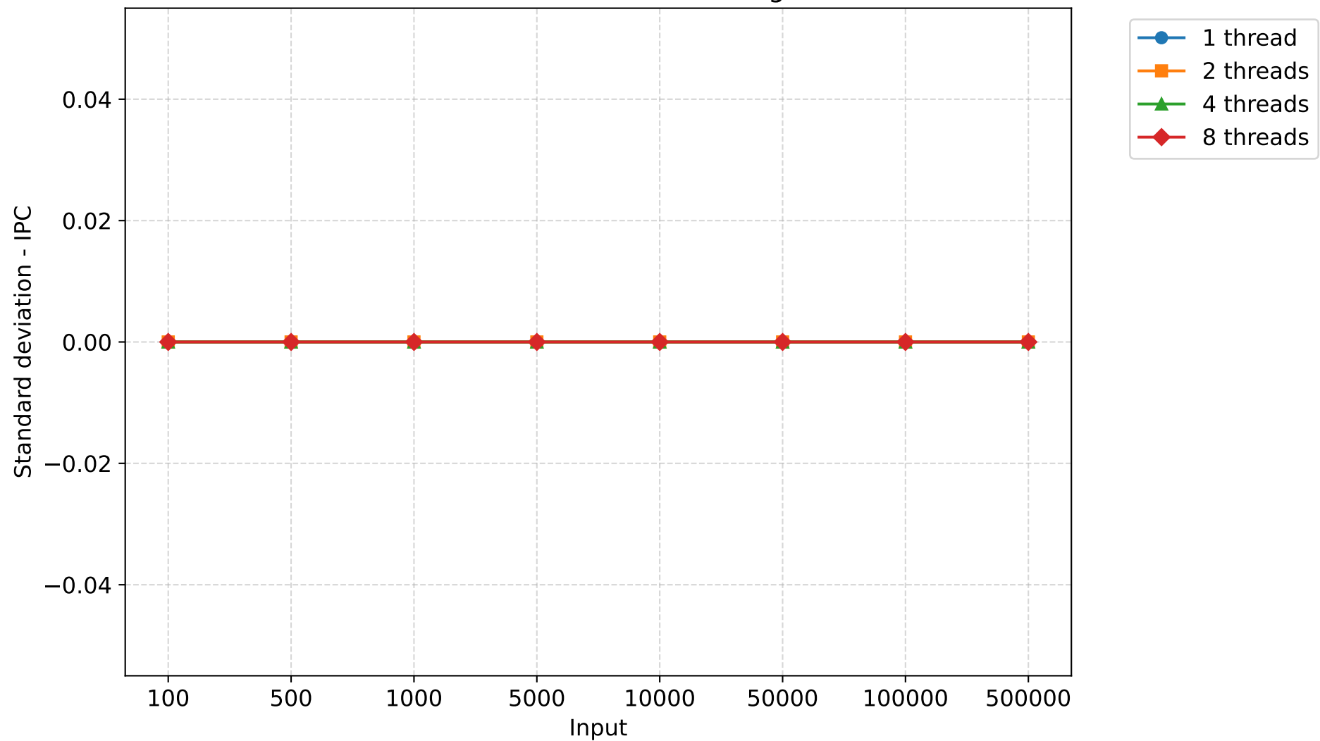
Standard deviation of IPC - mergesort
