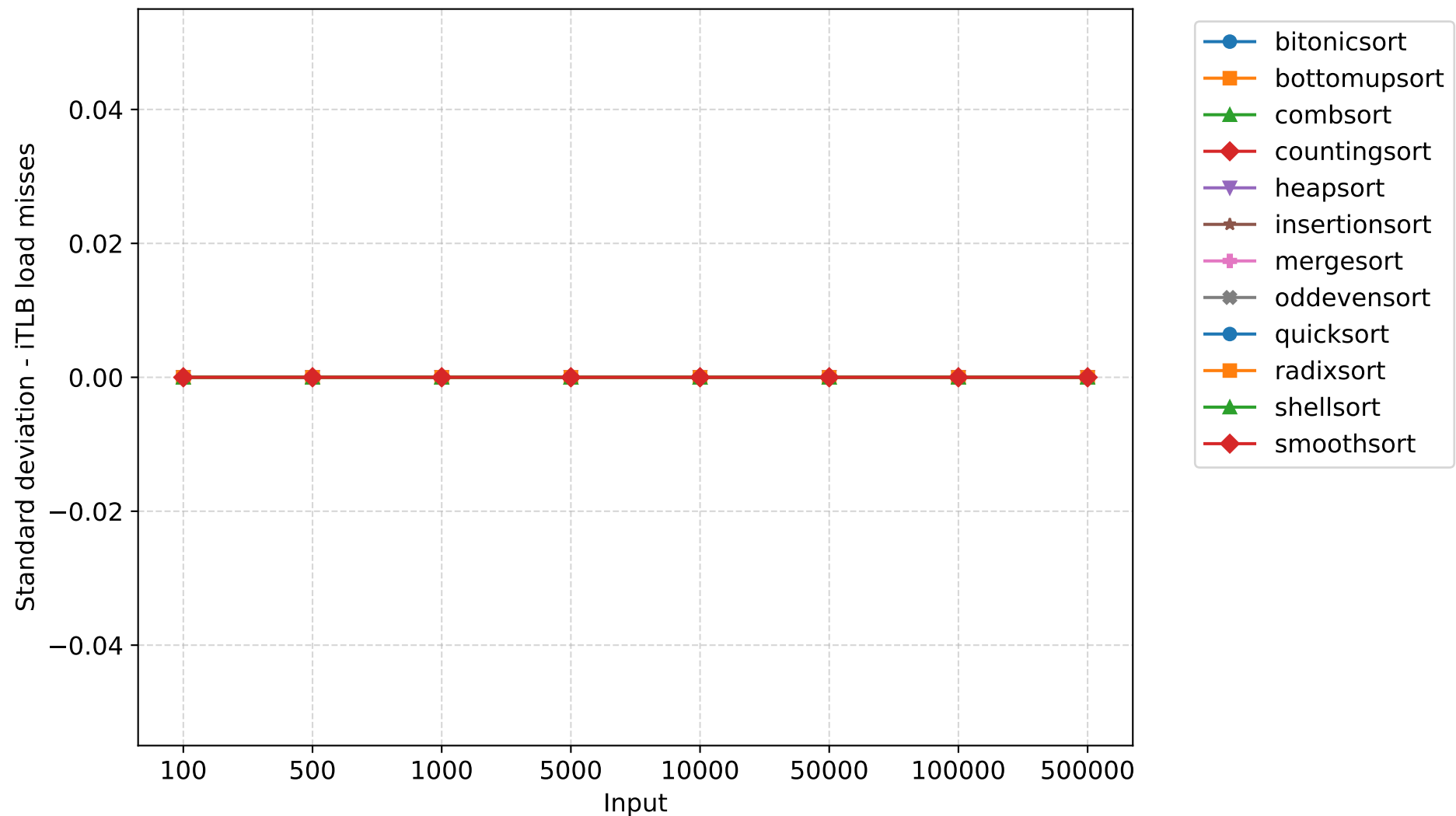
Standard deviation of iTLB load misses - 2 threads
