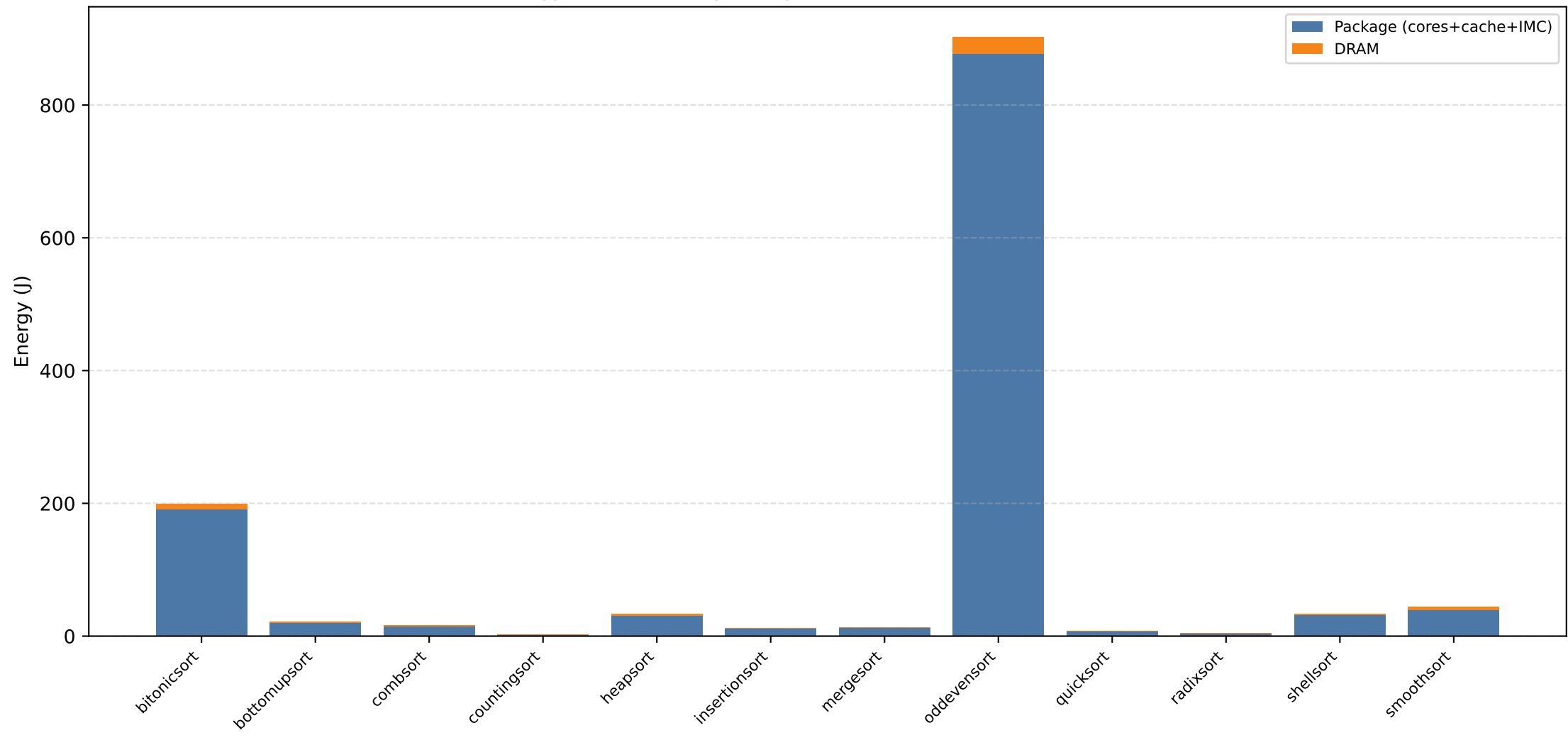
Energy breakdown: package vs DRAM (N=10000000, serial)
