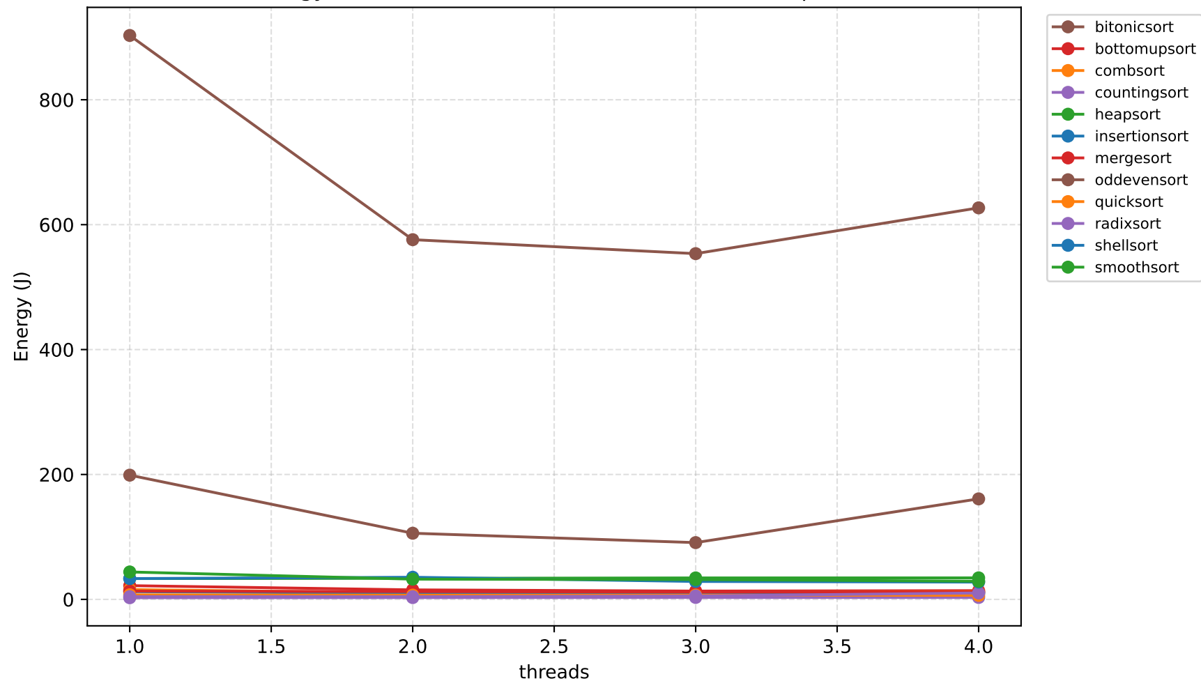
Total energy vs threads (N=10000000) — does not drop like time
