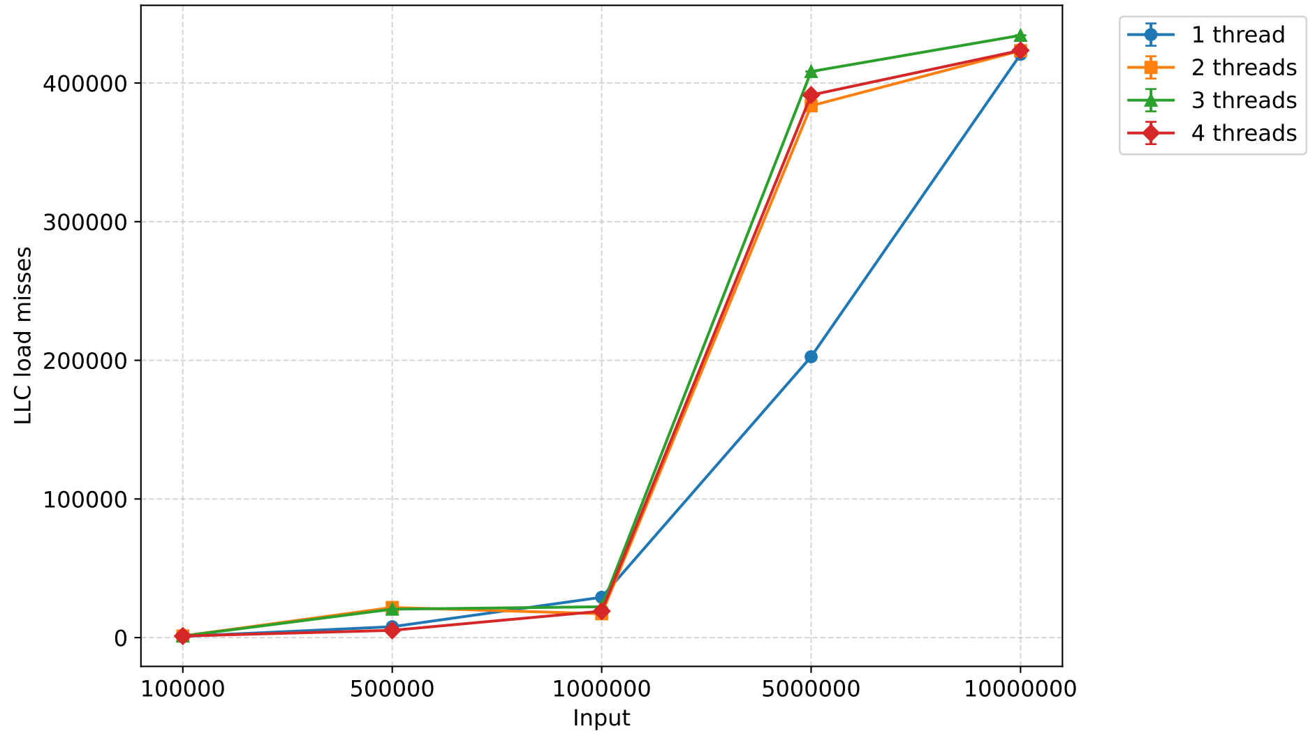
LLC load misses - bottomupsort (mean \pm 95% CI)
