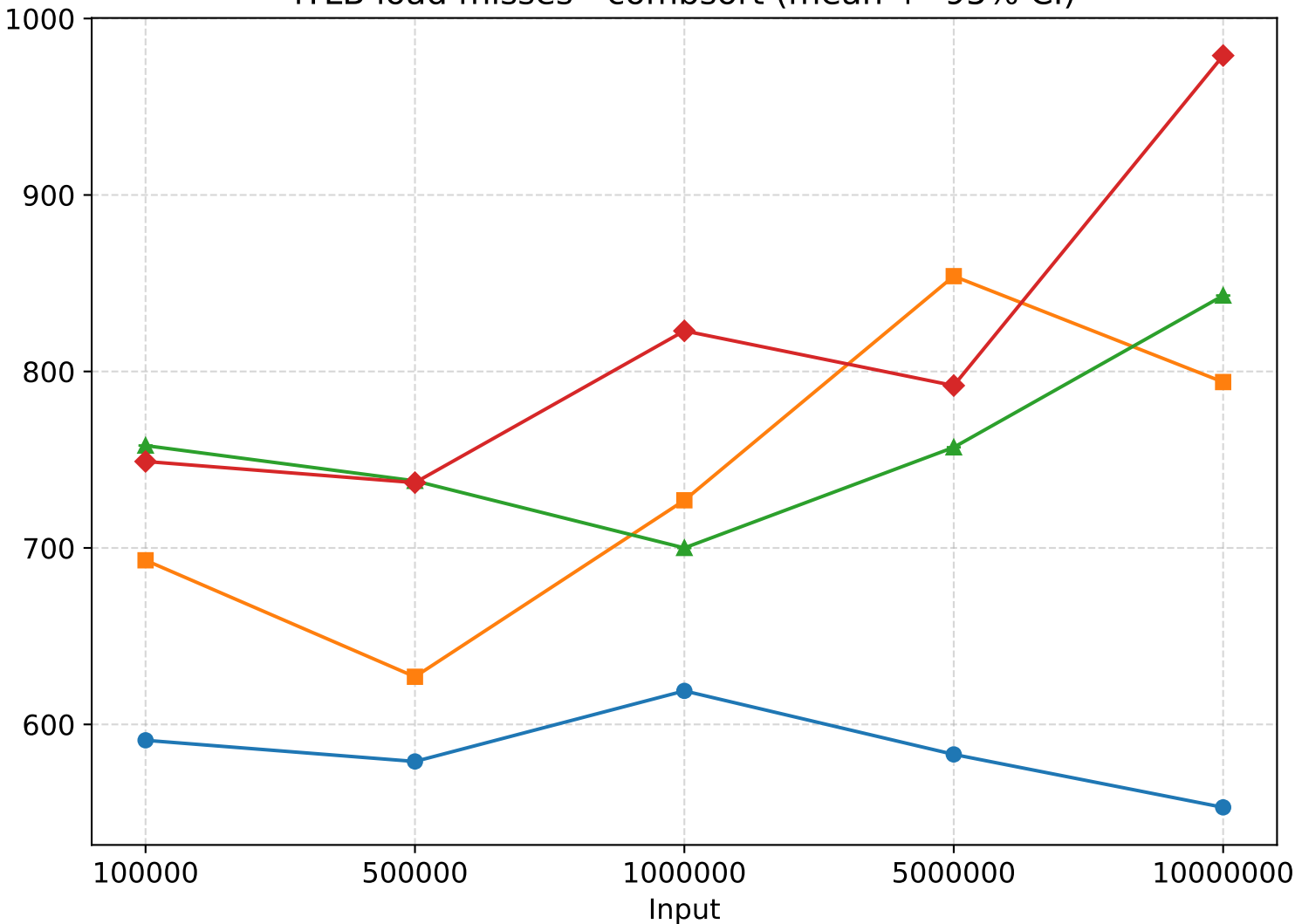
iTLB load misses - combort (mean \pm 95% CI)
