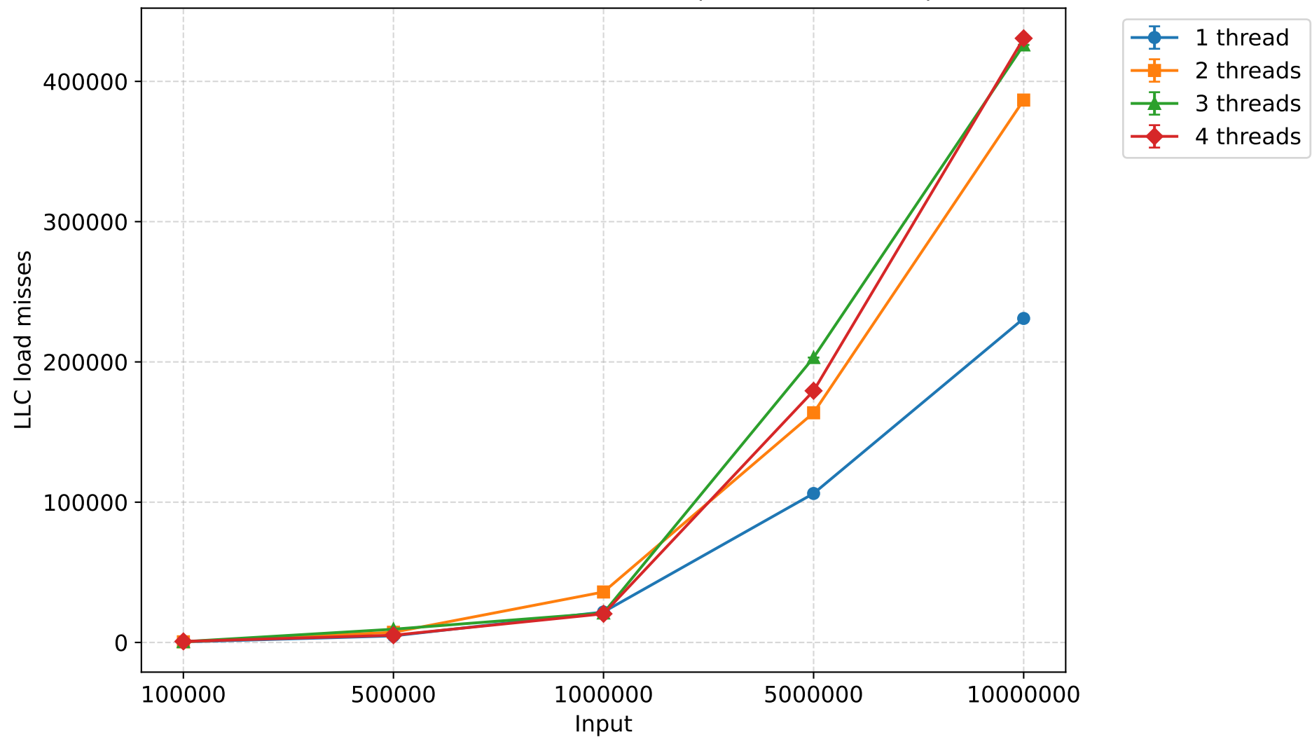
LLC load misses - insertion sort (mean \pm 95% CI)
