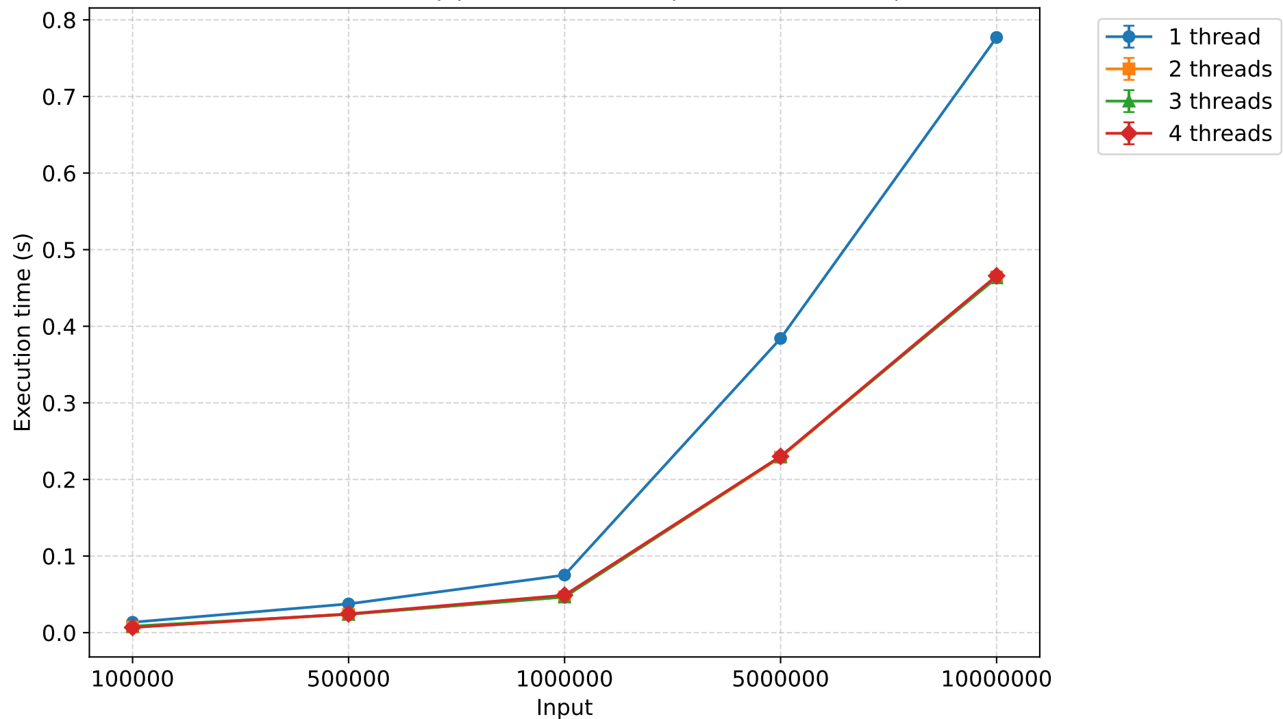
Execution time (s) - insertion sort (mean \pm 95% CI)
