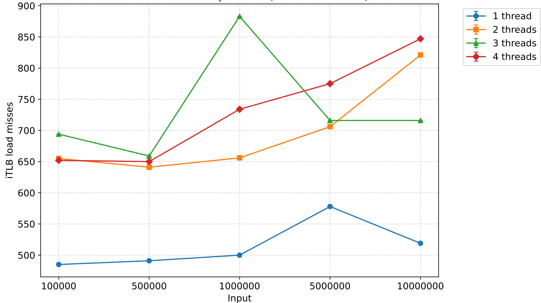
iTLB load misses - quicksort (mean \pm 95% CI)
