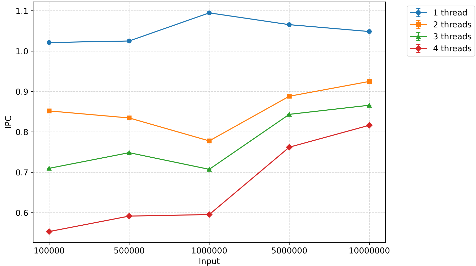
IPC - quicksort (mean \pm 95% CI)
