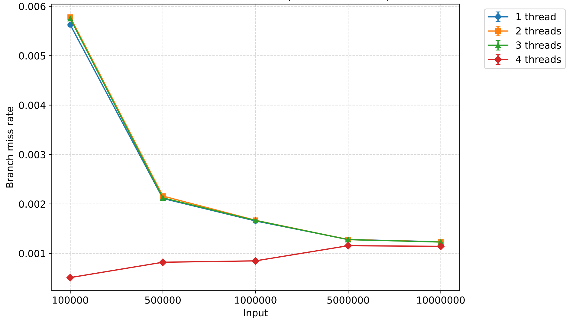
Branch miss rate - radixsort (mean \pm 95% CI)
