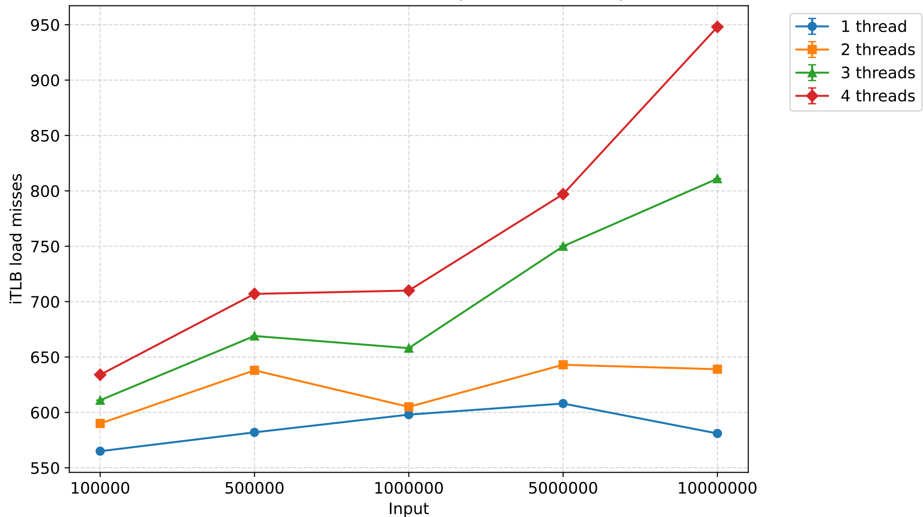
iTLB load misses - shellsort (mean \pm 95% CI)
