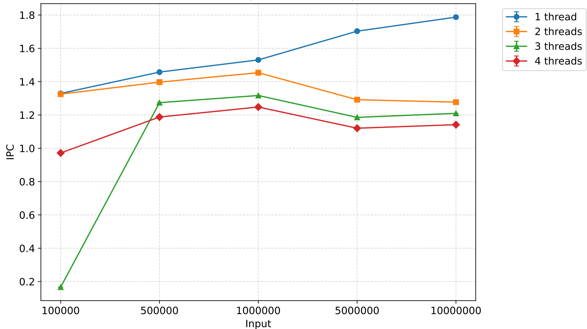
IPC - shellsort (mean \pm 95% CI)
