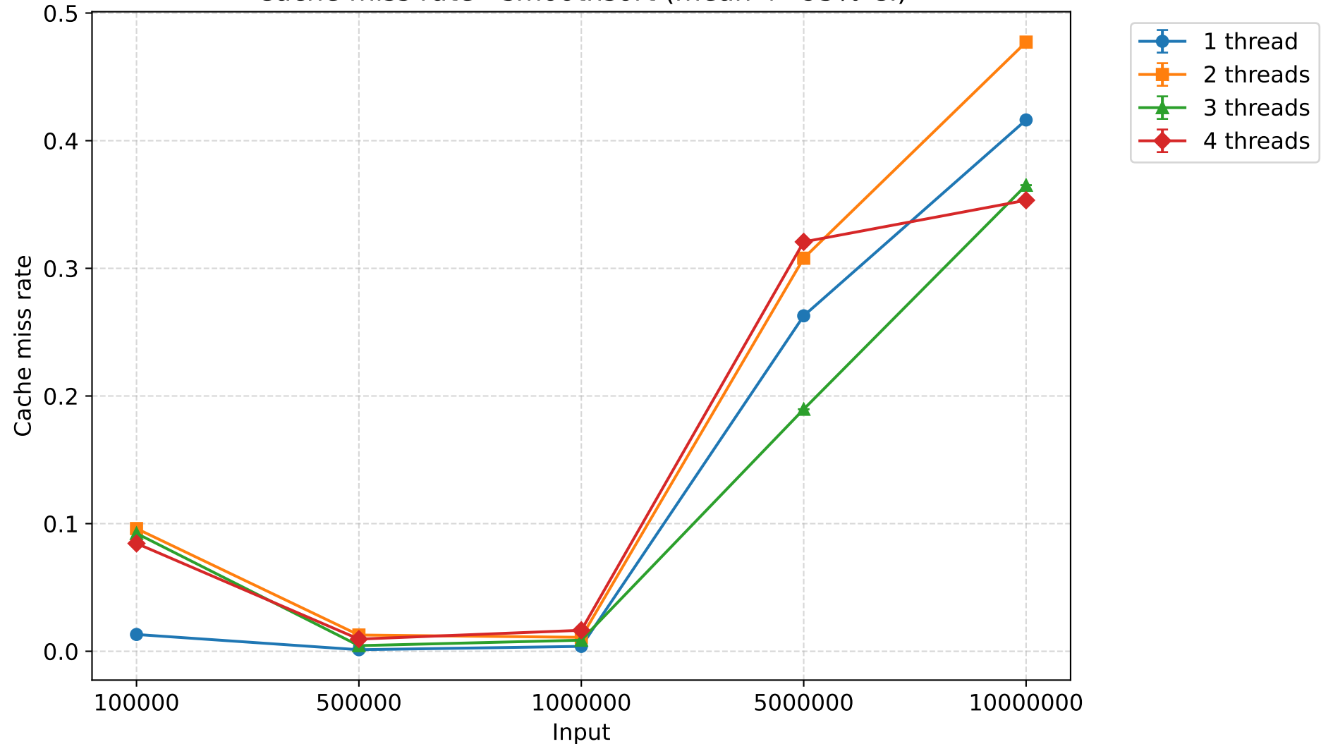
Cache miss rate - smoothsort (mean \pm 95% CI)
