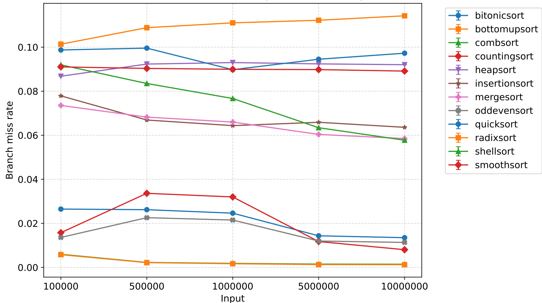
Branch miss rate - 2 threads (mean \pm 95% CI)
