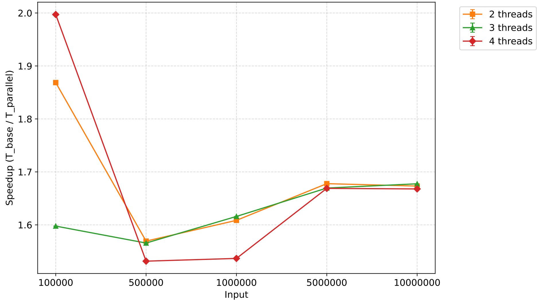
Speedup - insertionsort (mean \pm 95% CI)
