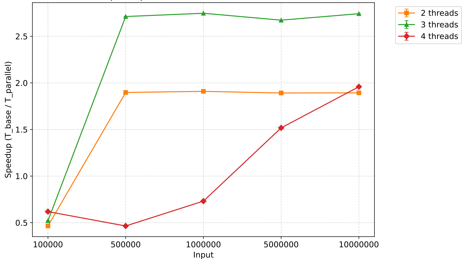
Speedup - oddevensort (mean \pm 95% CI)
