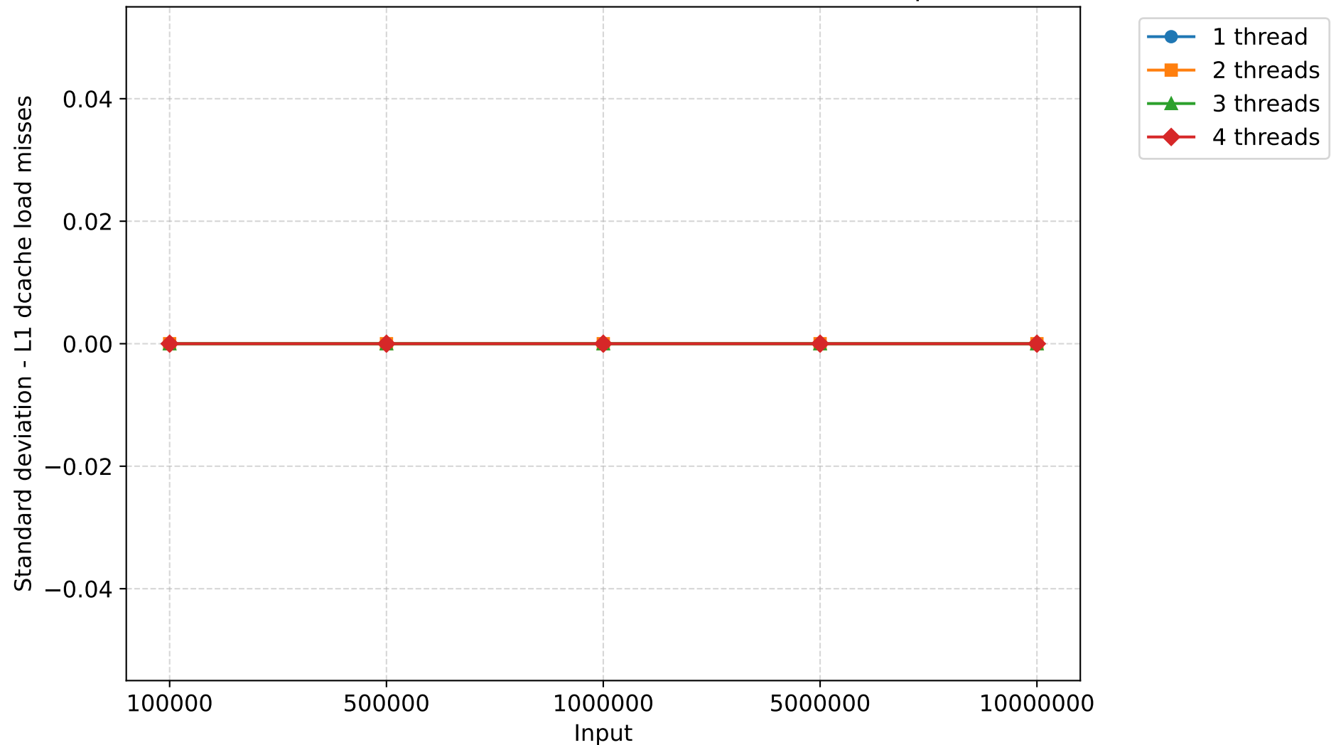
Standard deviation of L1 dcache load misses - heapsort
