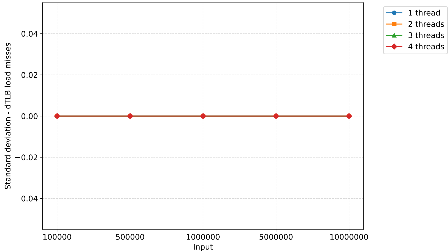
Standard deviation of dTLB load misses - smoothsort
