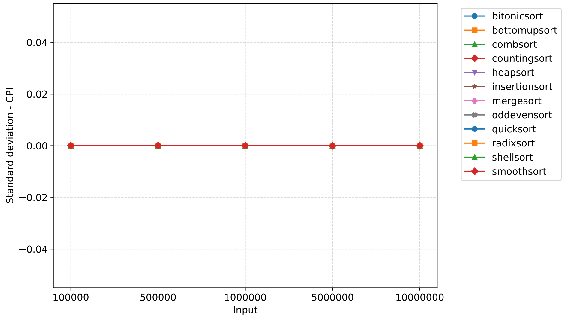
Standard deviation of CPI - 2 threads
