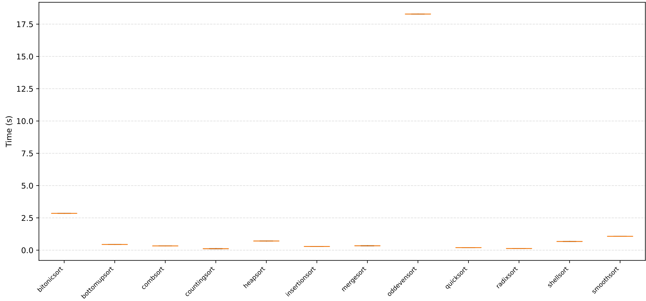
Distribution over repetitions ( N = 5000000 , serial)
