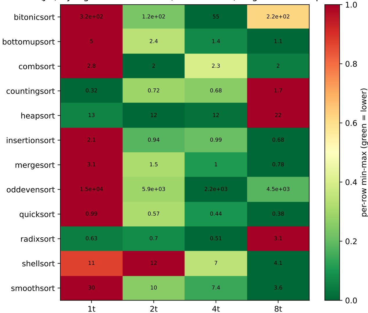
EDP (J·s) by algorithm x threads ( N = 5000000 ) — green = best per row
