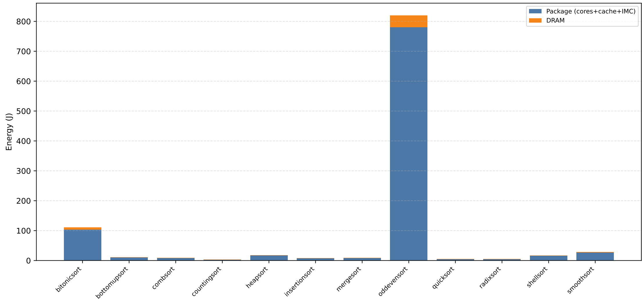
Energy breakdown: package vs DRAM ( N = 5000000 , serial)
