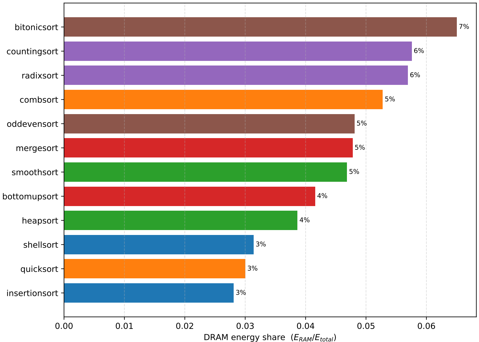
Share of energy spent in DRAM ( N = 5000000 , serial) — higher = more memory-bound
