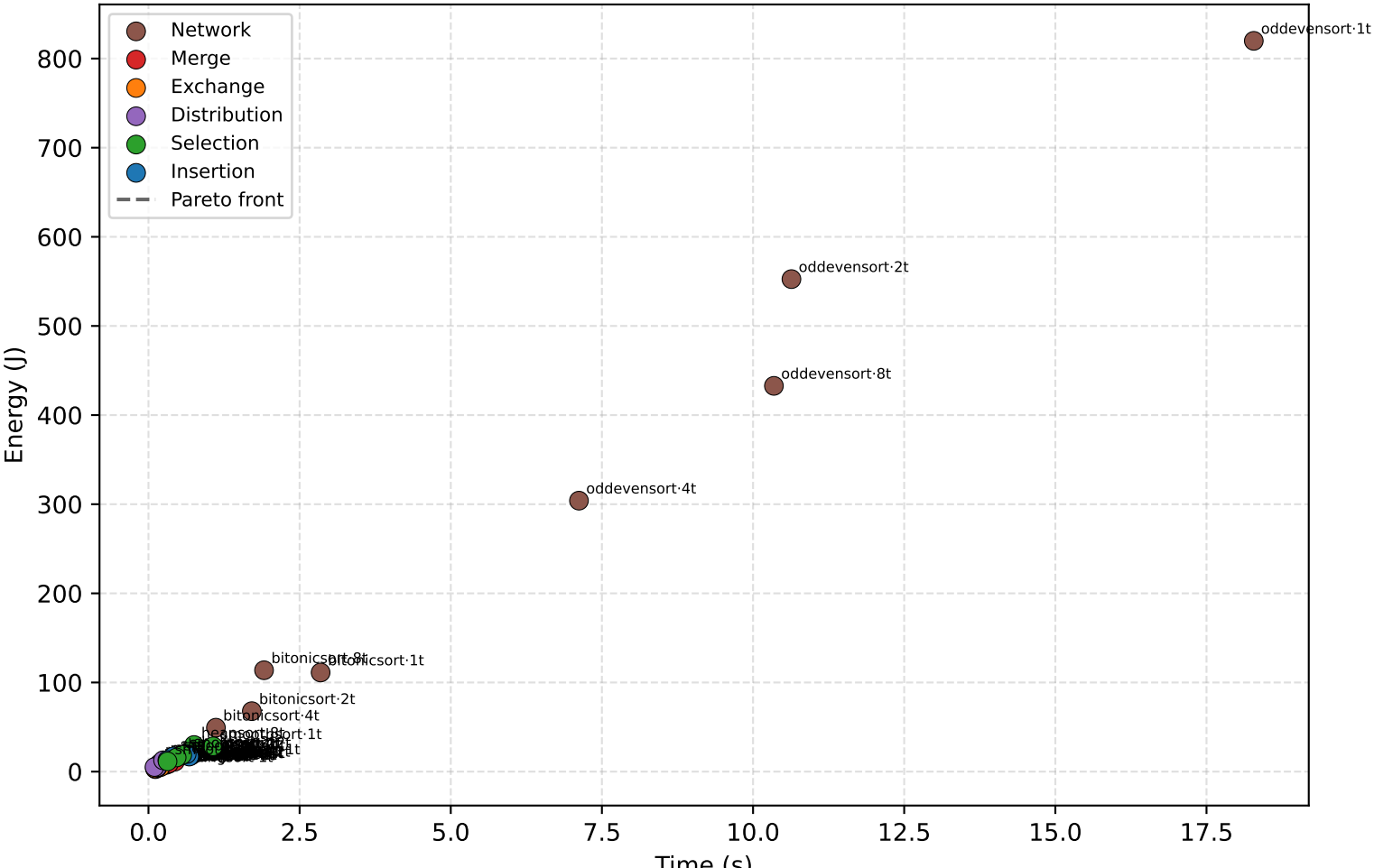
Energy-time trade-off ( N = 5000000 , all thread counts)
