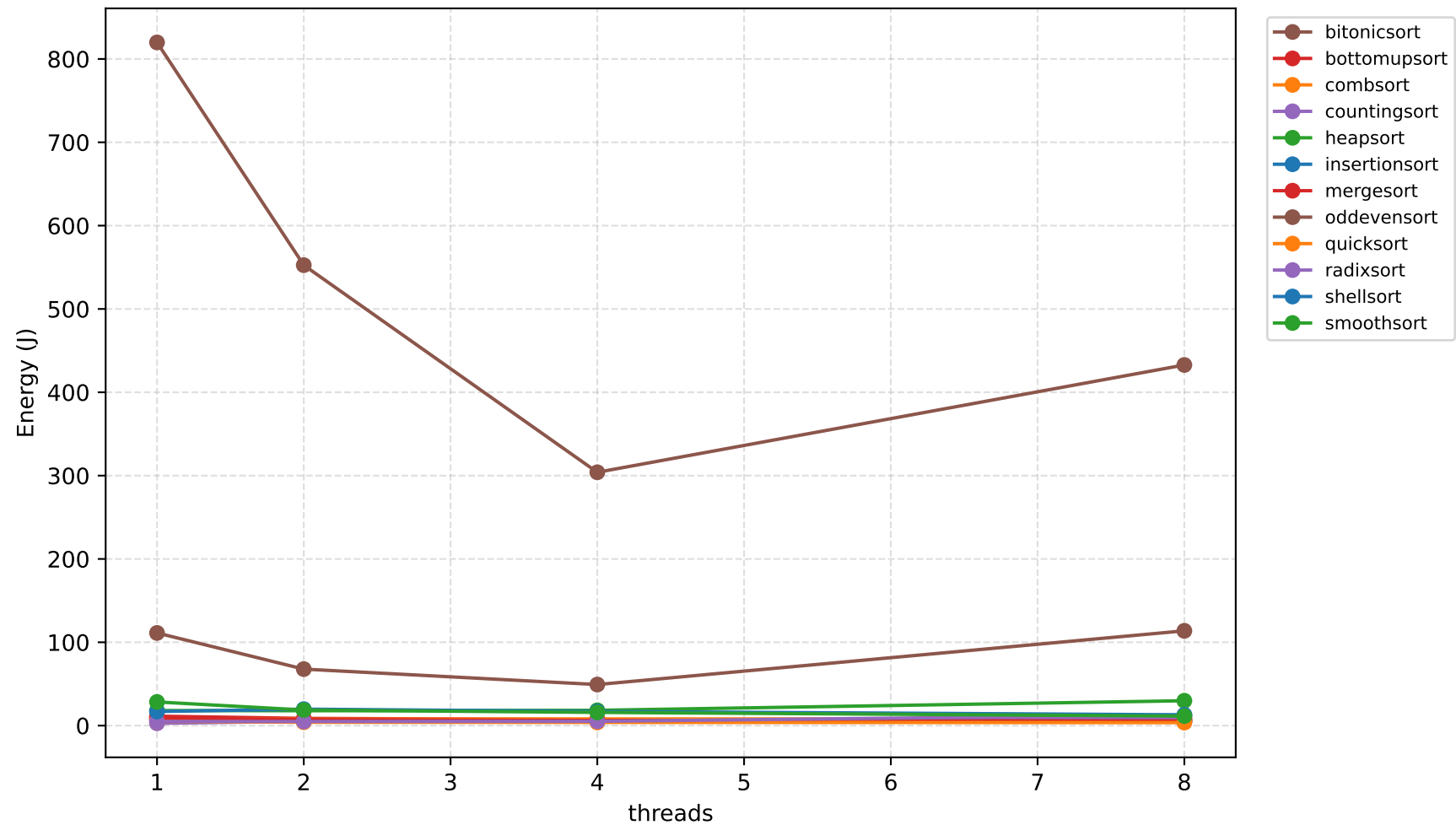
Total energy vs threads ( N = 5000000 ) — does not drop like time
