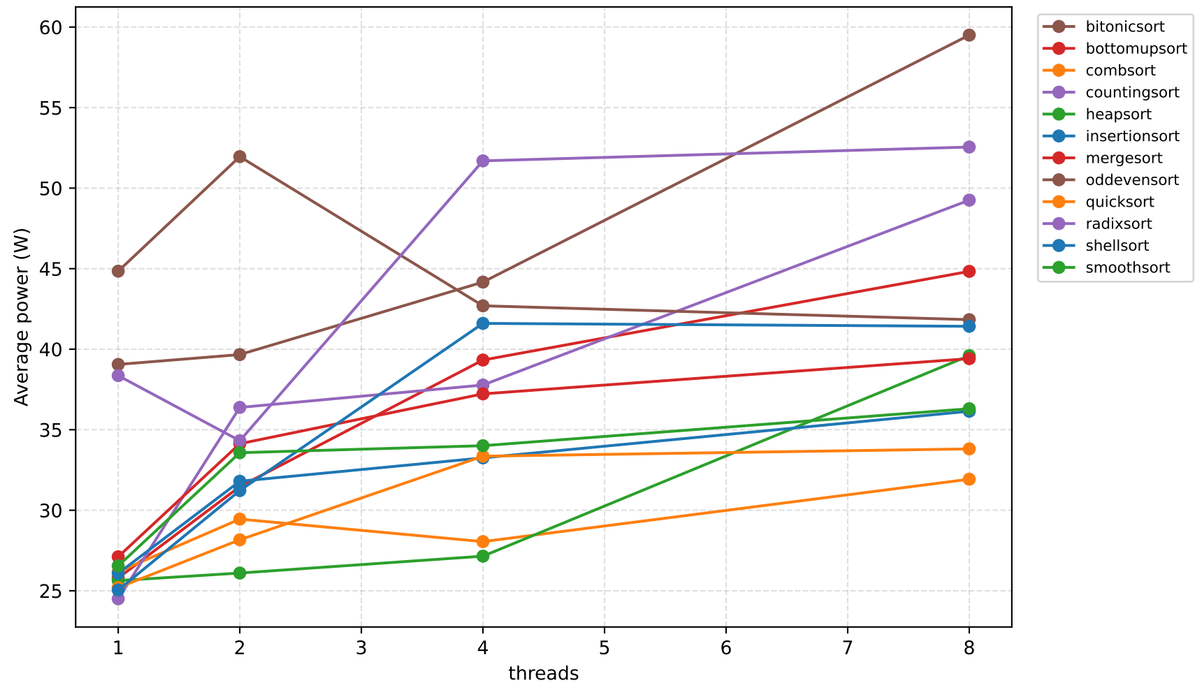
Average power vs threads ( N = 5000000 ) — rises with active cores
