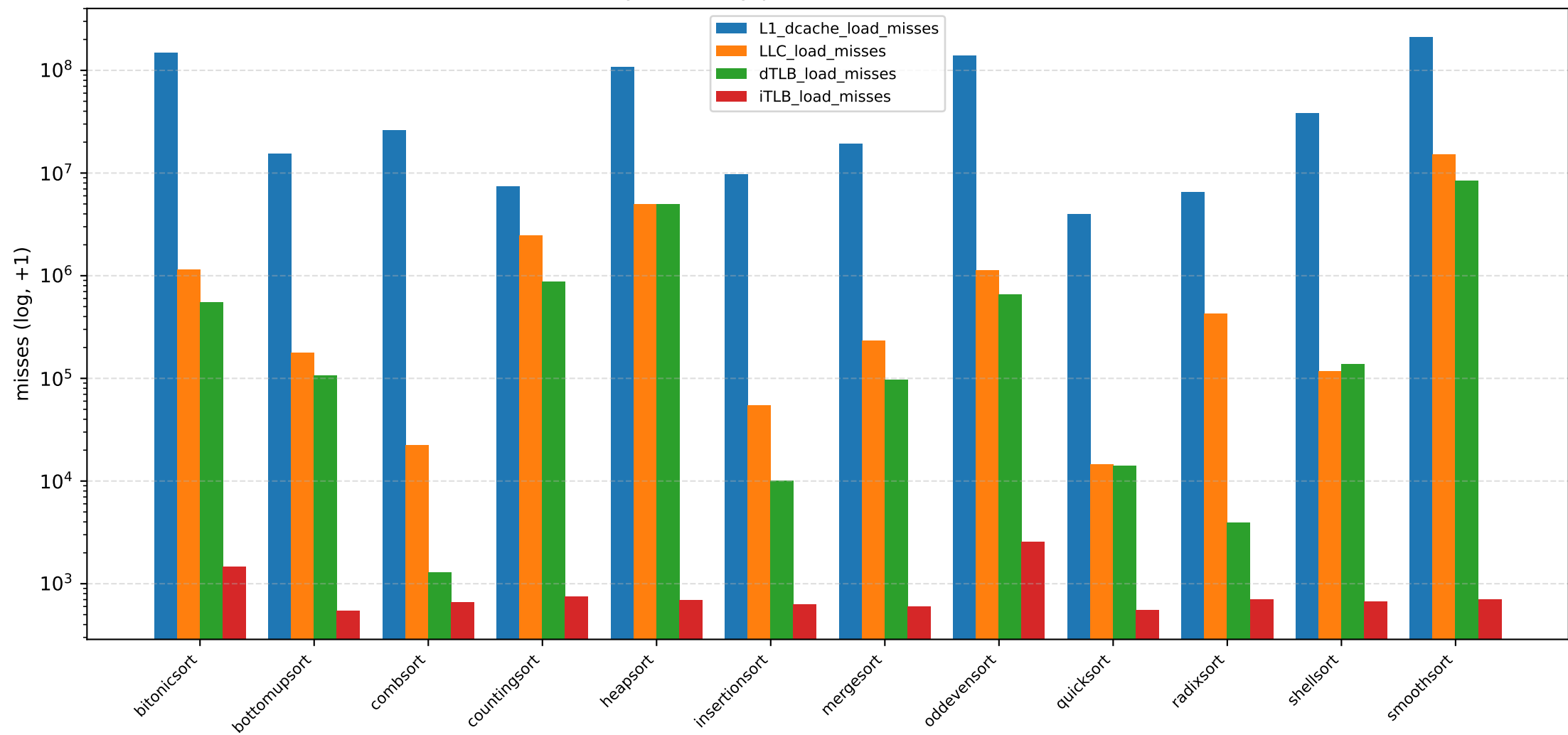
Memory hierarchy pressure ( N = 5000000 , serial)
