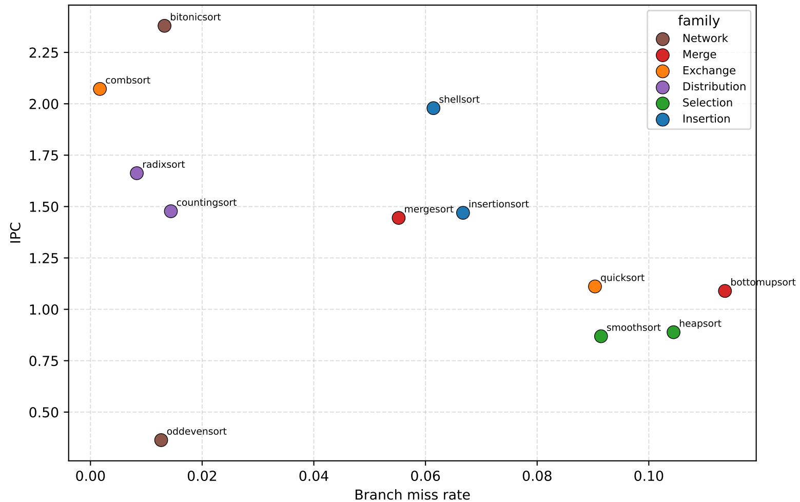
Microarchitecture fingerprint ( N = 5000000 , serial)
