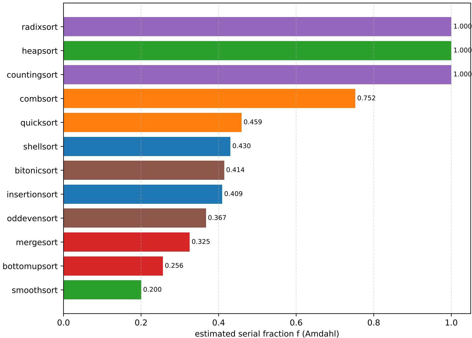
Serial fraction per algorithm ( N = 5000000 ) — lower f scales better
