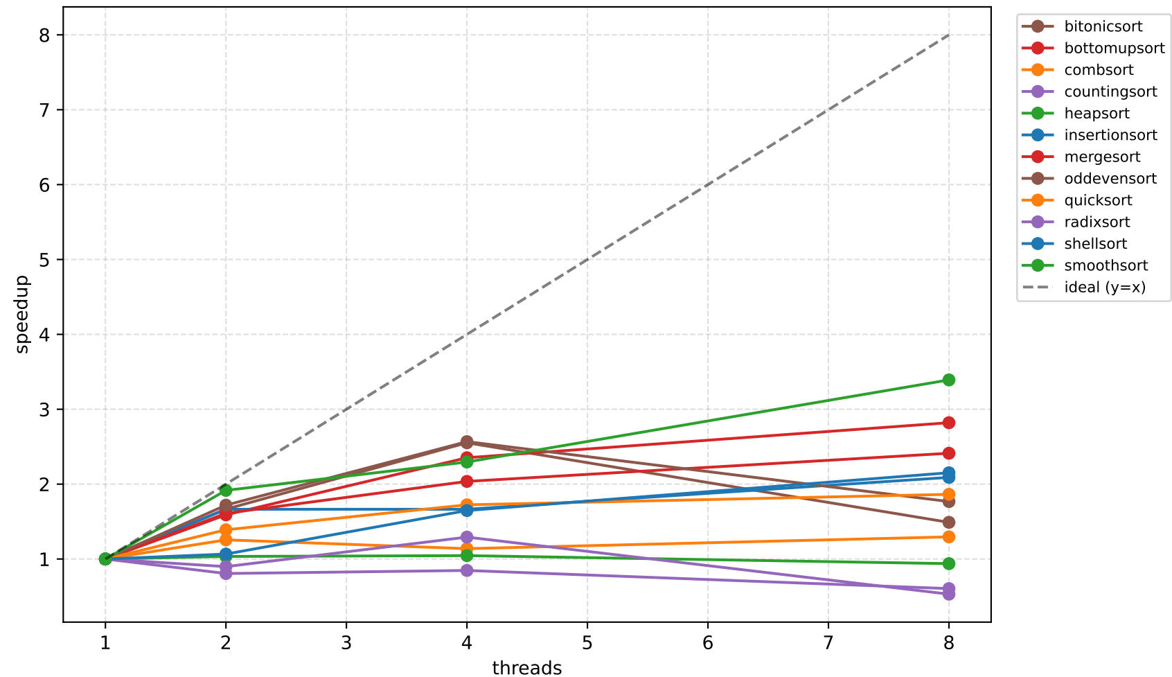
Speedup vs threads ( N = 5000000 ) with ideal line
