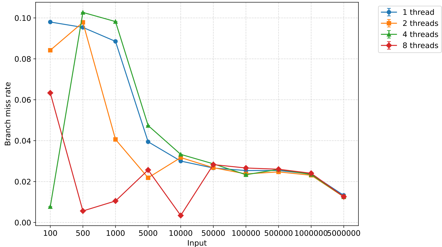
Branch miss rate - bitonicsort (mean \pm 95% CI)
