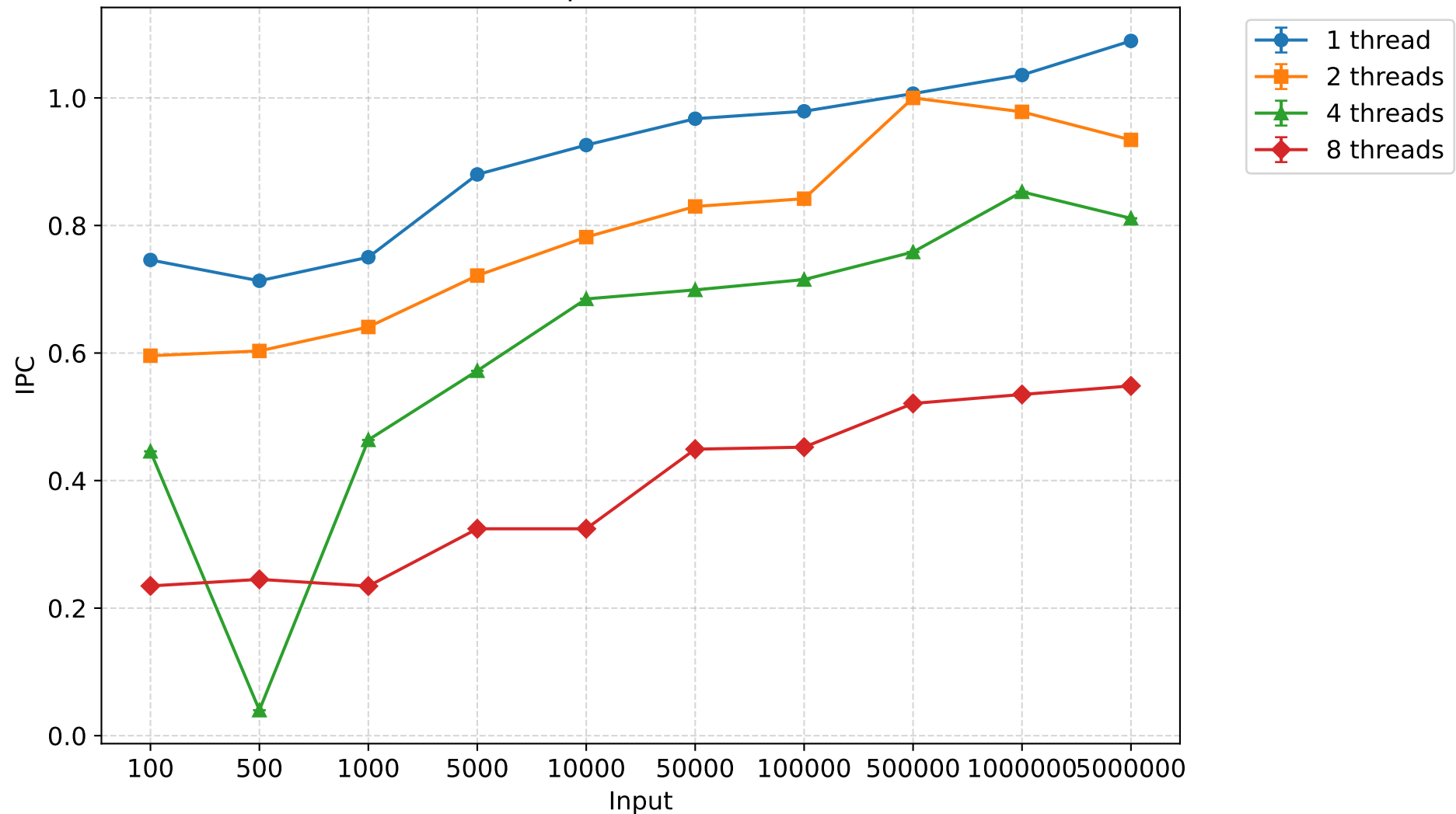
IPC - bottomupsort (mean \pm 95% CI)
