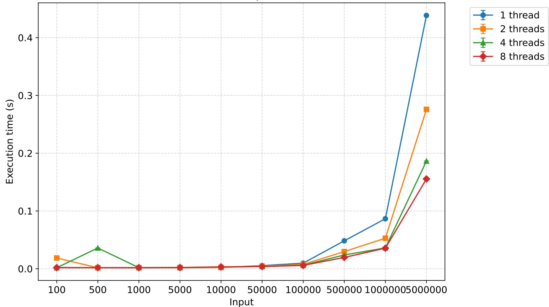
Execution time (s) - bottomupsort (mean \pm 95% CI)
