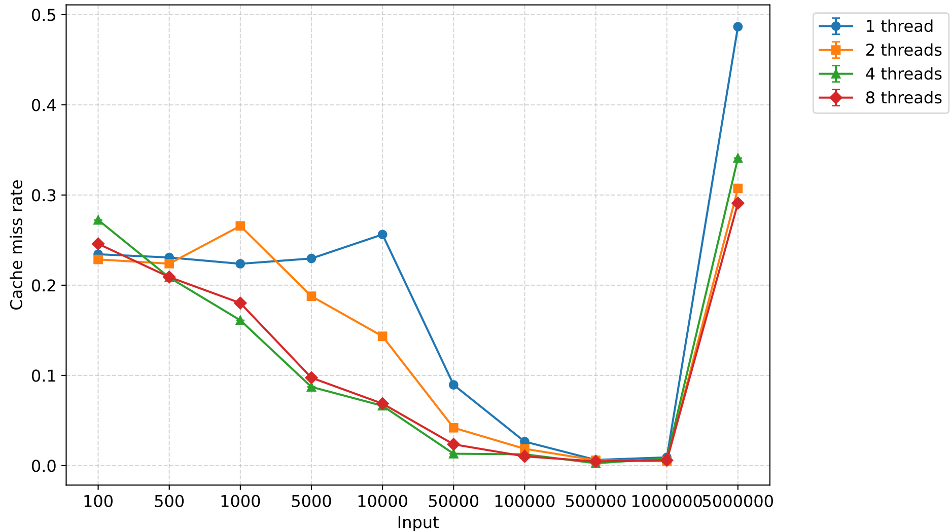
Cache miss rate - combsort (mean \pm 95% CI)
