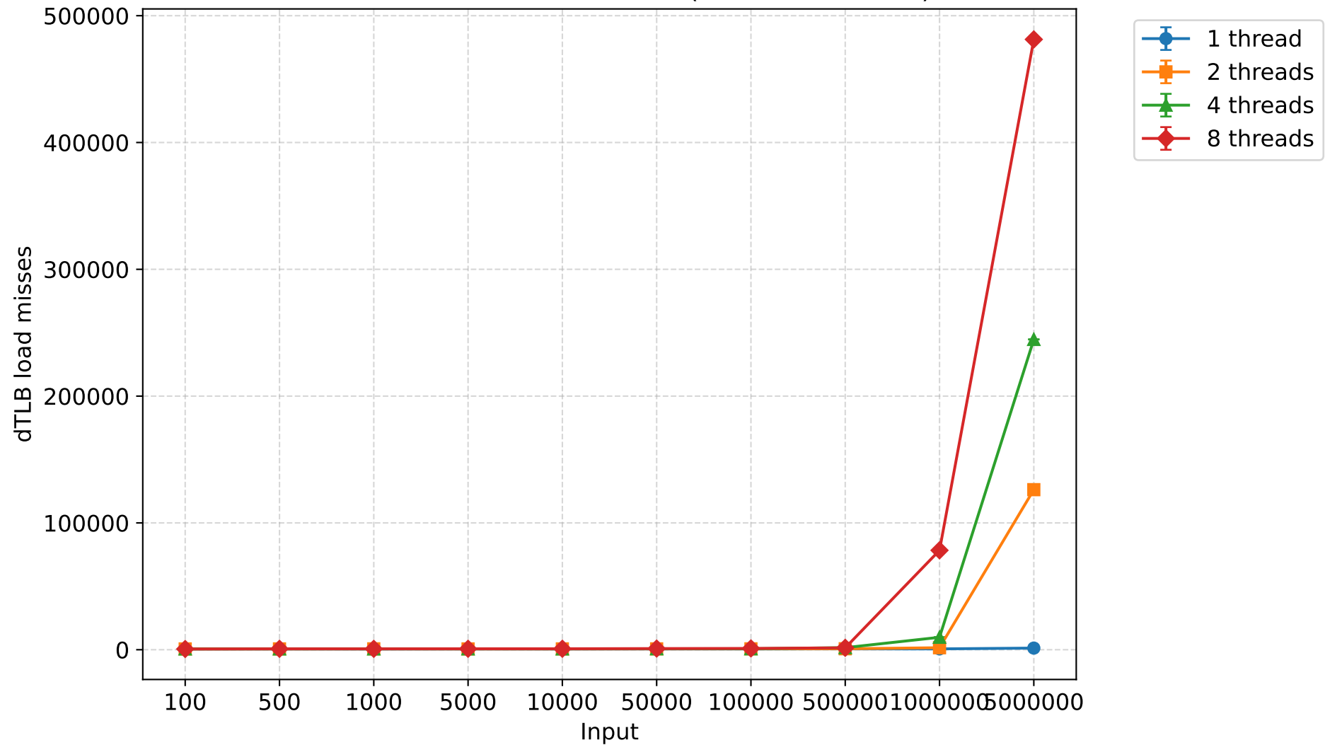
dTLB load misses - combSort (mean \pm 95% CI)
