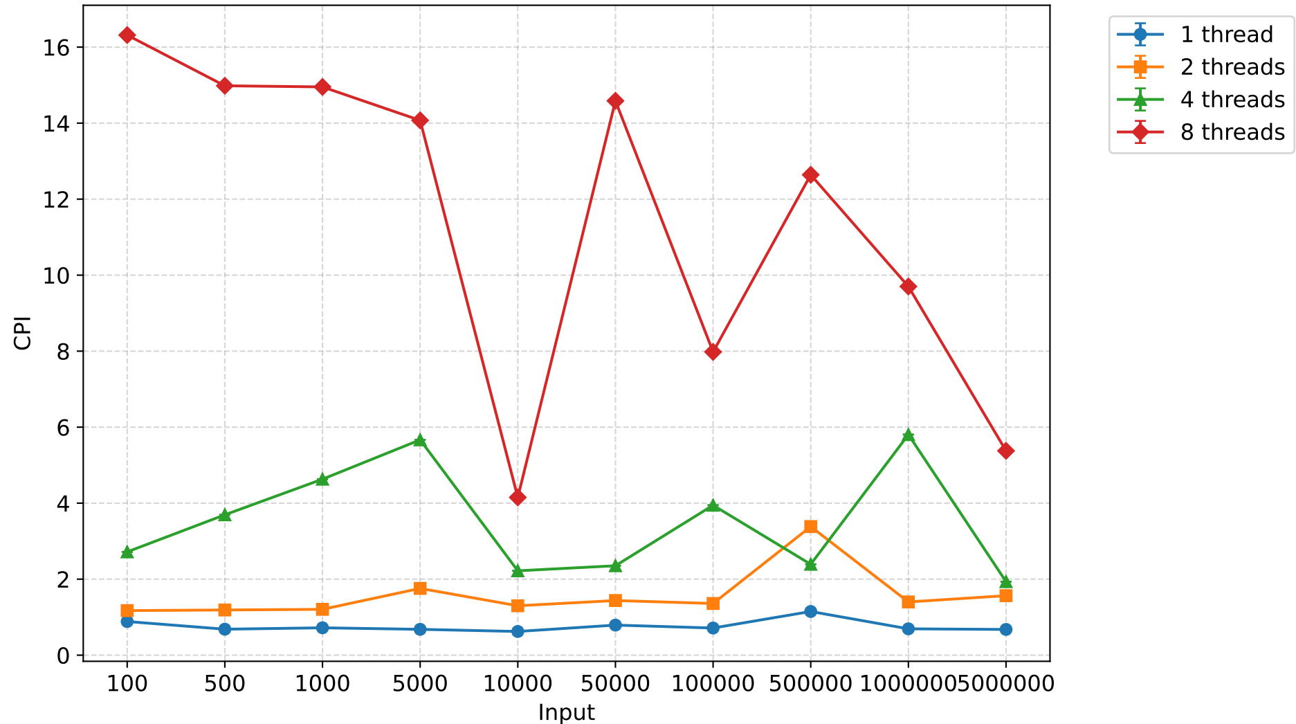
CPI - counting sort (mean \pm 95% CI)
