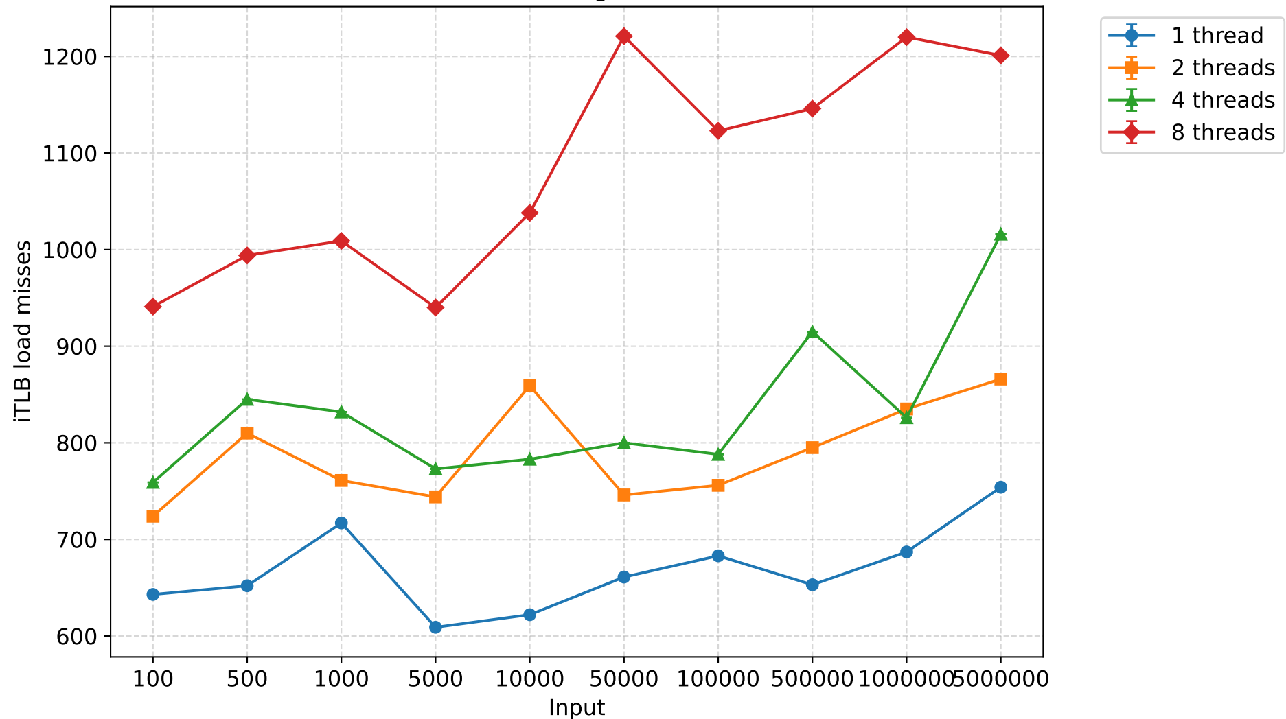
iTLB load misses - counting sort (mean \pm 95% CI)
