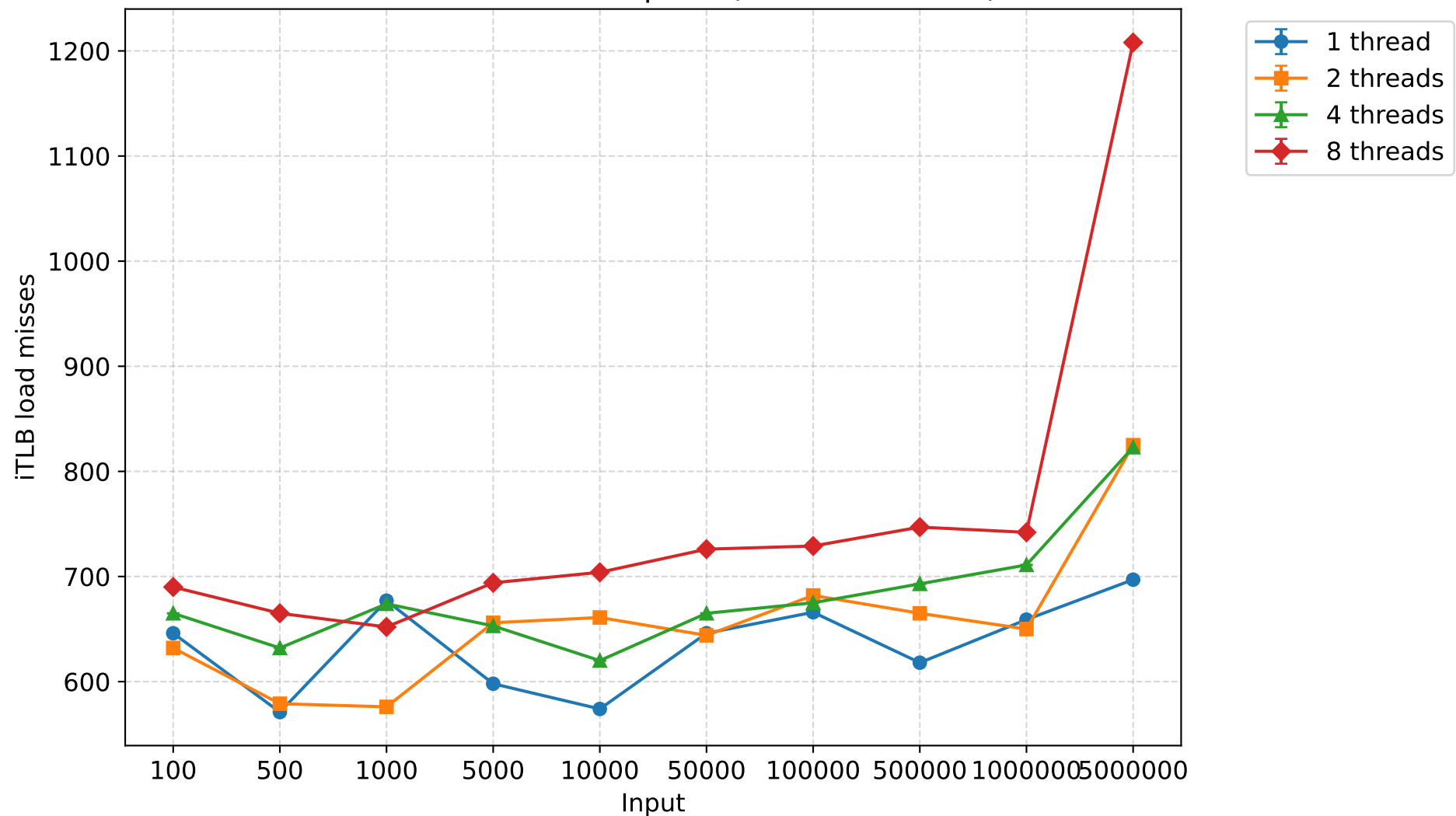
iTLB load misses - heapsort (mean \pm 95% CI)
