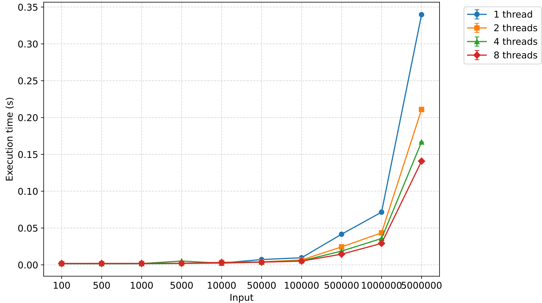
Execution time (s) - mergesort (mean \pm 95% CI)
