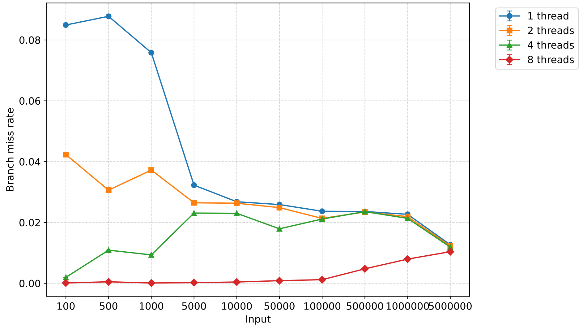
Branch miss rate - oddevensort (mean \pm 95% CI)
