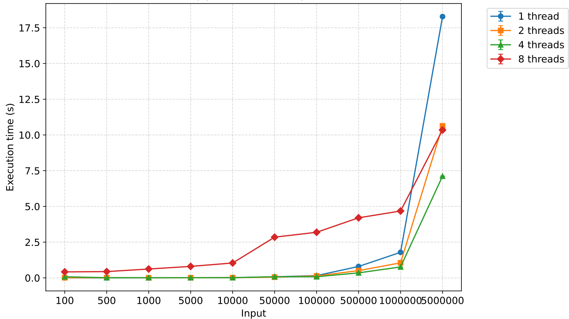
Execution time (s) - oddevensort (mean \pm 95% CI)
