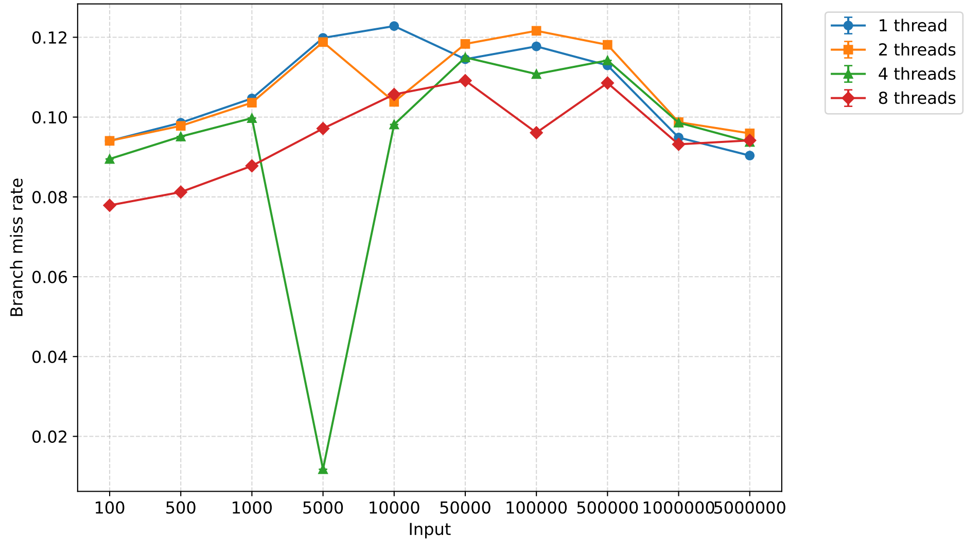
Branch miss rate - quicksort (mean \pm 95% CI)
