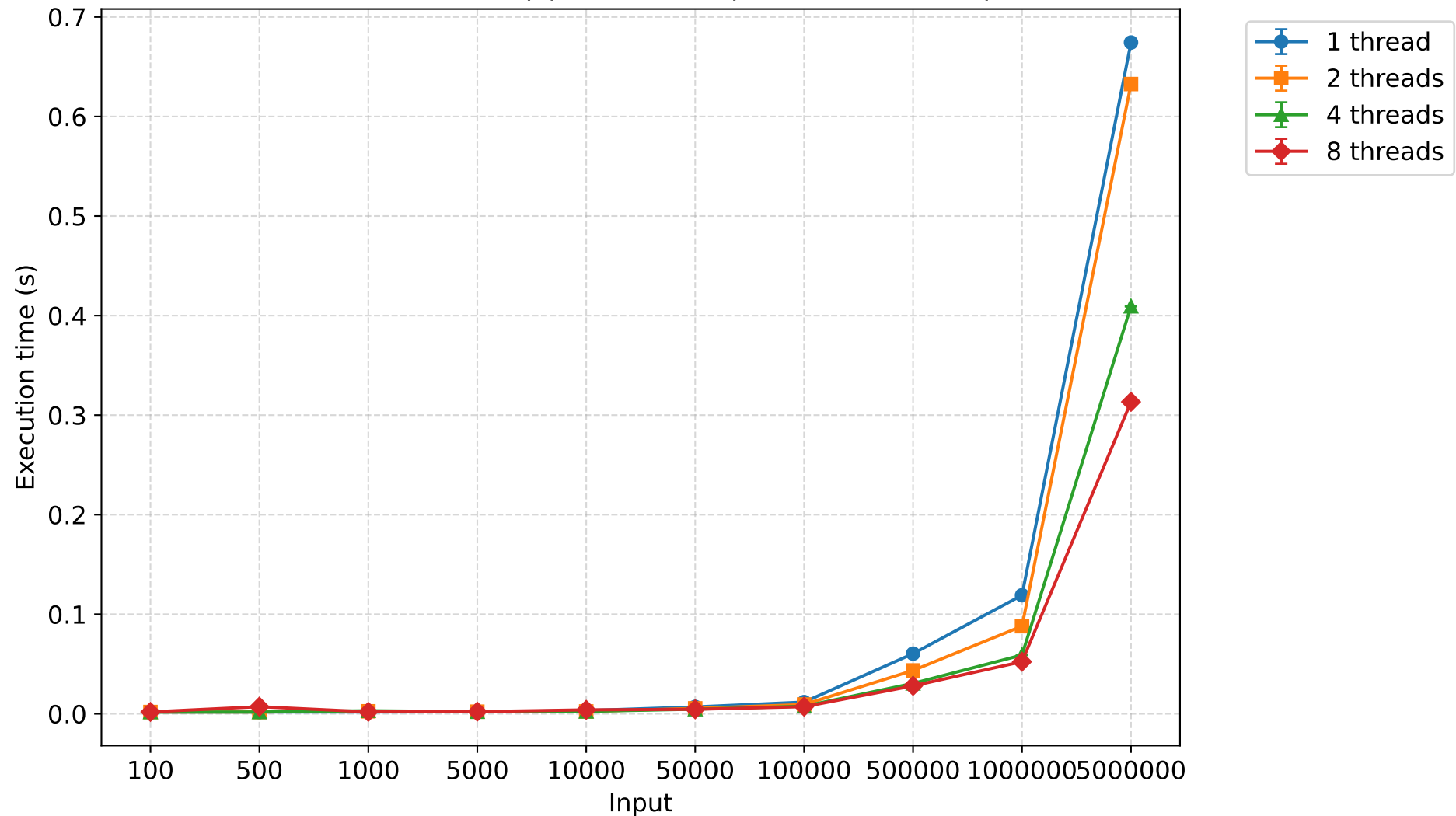
Execution time (s) - shellsort (mean \pm 95% CI)
