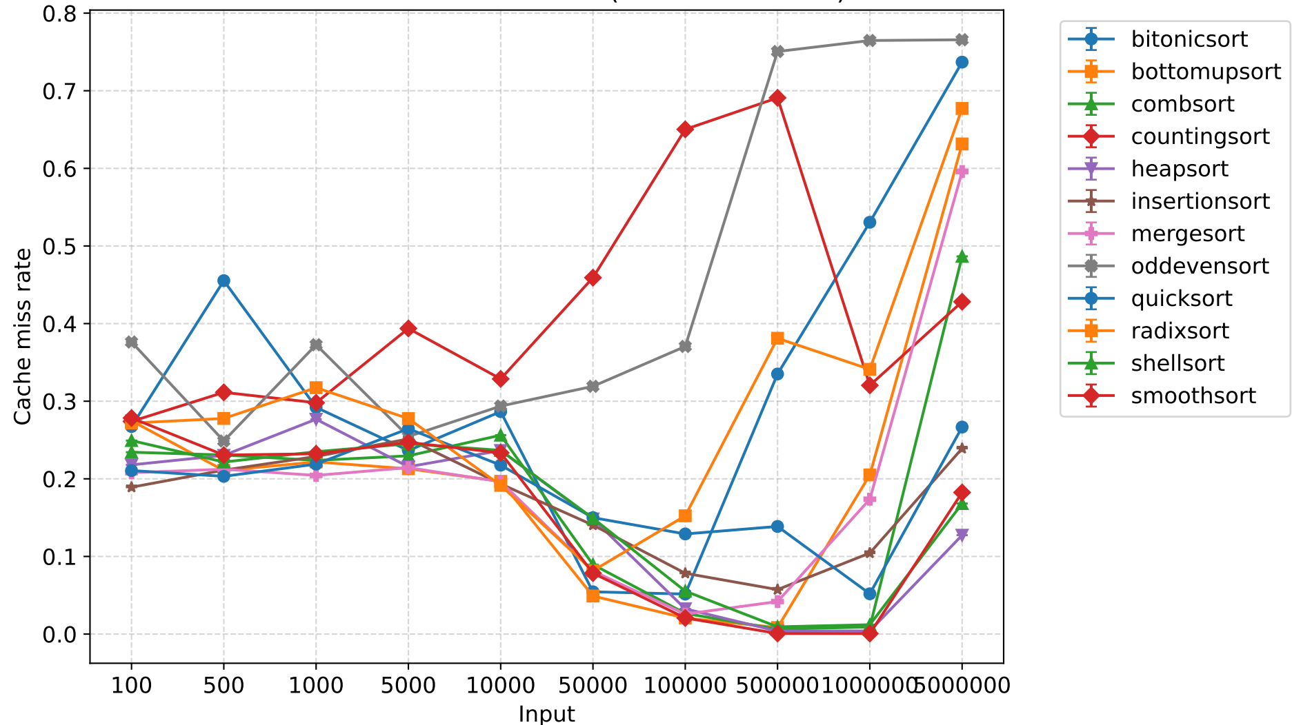
Cache miss rate - 1 thread (mean \pm 95% CI)
